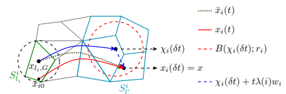
Fig. 2. Illustration of the reference trajectory and reachability capabilities of the control laws.
