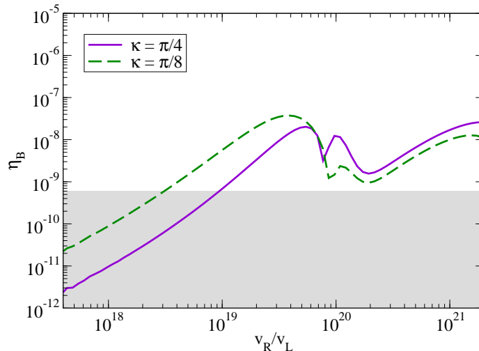
Figure 11: The baryon-to-photon ratio \eta_B with an additional complex phase \pi/8 or \pi/4 attributed to the electron neutrino for the solution ‘--+’. The shaded area corresponds to values of \eta_B below the observed value. Inverted mass hierarchy, m_0 = 0.1 eV.
