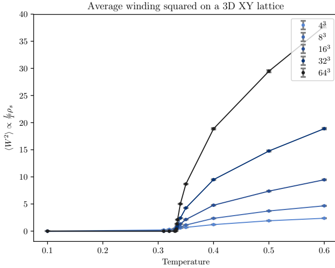
Figure 4.7: Average winding number squared, \langle W^2 \rangle \propto \rho_s , plotted on a 3D XY lattice of varying sizes. The overall structure of the average winding number squared as a function of the temperature is shown.
