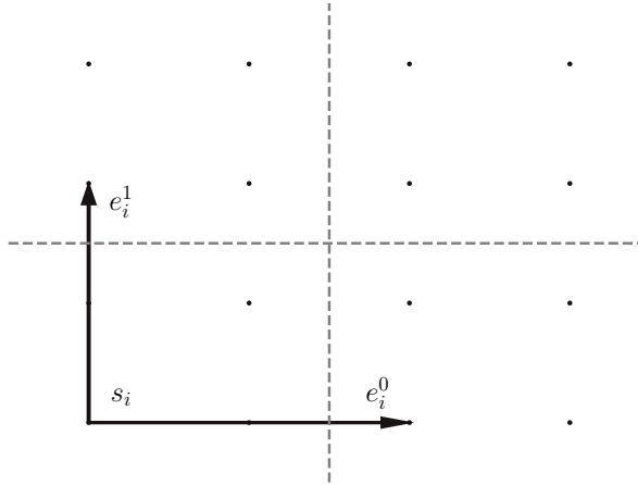
Figure 3.1: One step in the graph dividing algorithm where l_i = 4 . e_i^0 and e_i^1 are drawn from site s_i . Summed permutations of \{e_i^0, e_i^1\} give the starts for the next boxes. The next iteration of boxes are shown via the dividing dotted lines.
