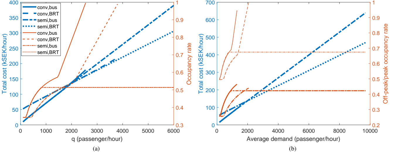
Figure 10.: Results of total cost and occupancy rate with respect to (a) demand q (one-period analysis) and (b) average demand \bar{q} (two-period analysis). Bus headway is restricted to no less than 3 minutes and BRT headway is restricted to no less than 2 minutes, q_2/q_1 = 3 , other parameters according to Table. 1. (a) and (b) share the line styles, except in (b) the wider occupancy rate lines are for off-peak hours and the thinner for peak hours.
