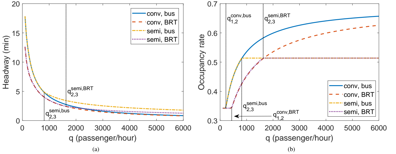
Figure 5.: Single-period results of (a) headway and (b) occupancy rate with respect to demand q , parameters according to Table. 1.
