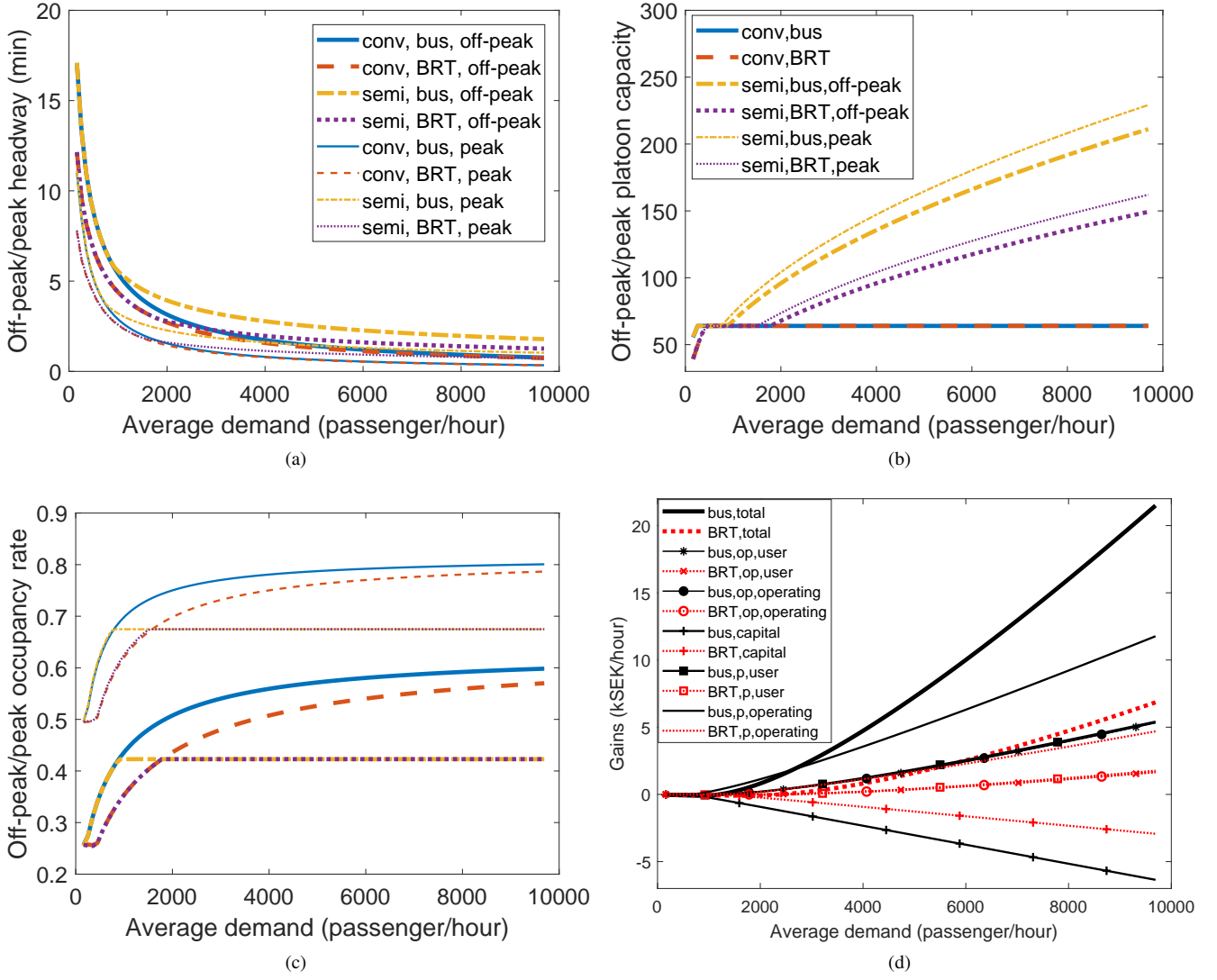
Figure 8.: Two-period results of (a) headway, (b) platoon capacity, (c) occupancy rate, and (d) gains of using semi-autonomous vehicles with respect to average demand \bar{q} , q_2/q_1 = 3 , other parameters according to Table. 1. (a) and (c) use the same line styles to distinguish different scenarios. In (d), 'p' is short for peak and 'op' is short for off-peak.
