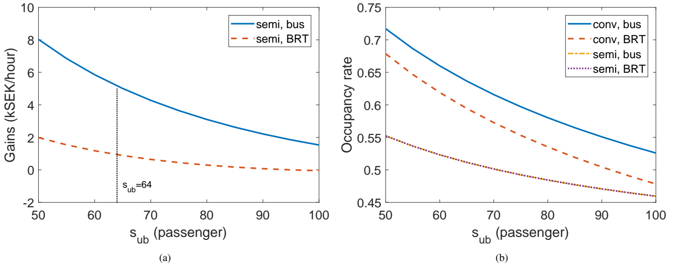
Figure 7.: Single-period results of (a) gains by using semi-autonomous vehicles and (b) occupancy rate with respect to capacity upper bound s_{ub} , parameters according to Table. 1.
