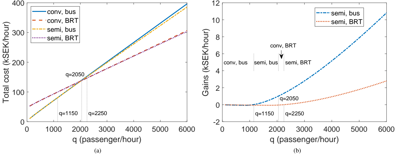
Figure 4.: Single-period results of total cost and gains from adopting semi-autonomous vehicles with respect to demand q , parameters according to Table. 1.
