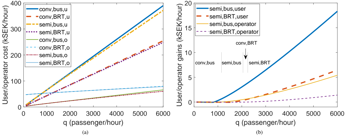
Figure 6.: Single-period results of (a) user cost and operator cost, (b) user gains and operator gains with respect to demand q , parameters according to Table. 1.
