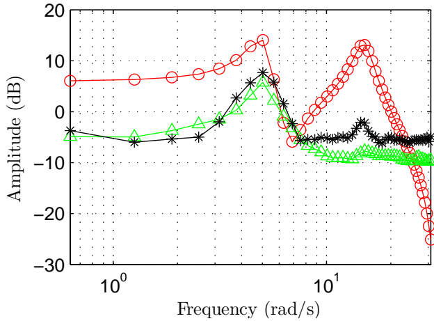
Fig. 3. Mean of the estimation error with noise for the proposed method ( -\triangle- ) and the local polynomial method ( -* - ). True frequency response G_0(e^{j\omega}) is shown as ( -\circ- ).
