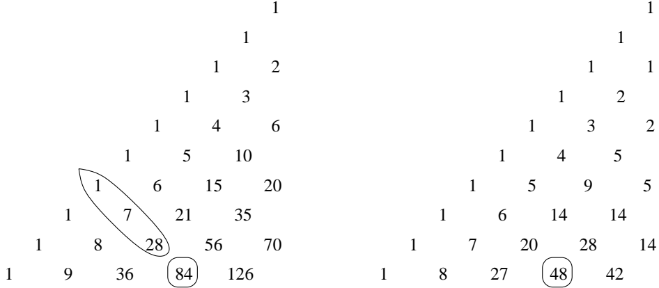
Figure B1. Pascal's triangle together with the coefficient triangle.
