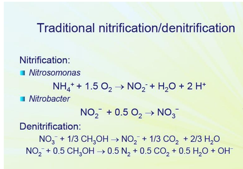
Fig. 2 Reaction of nitrification/denitrification.
