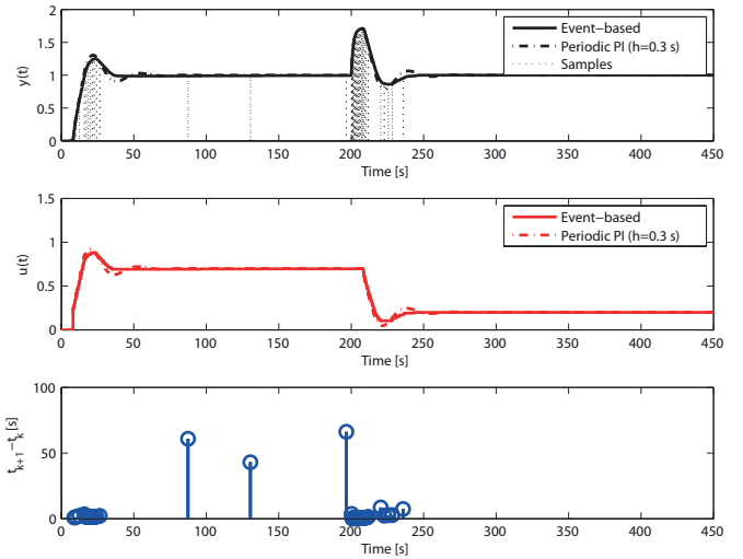
Fig. 6. Simulation result of a PIDPLUS controller with PI sampling for disturbance rejection under an actuation delay L = 8 s.
