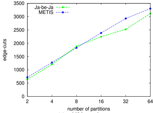
(a) add20 graph.
