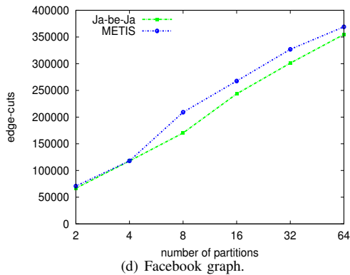
Figure 5. JA-BE-JA vs. METIS scalability in different graphs.
