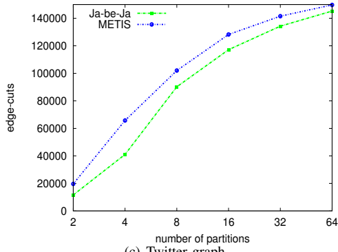
(c) Twitter graph.
