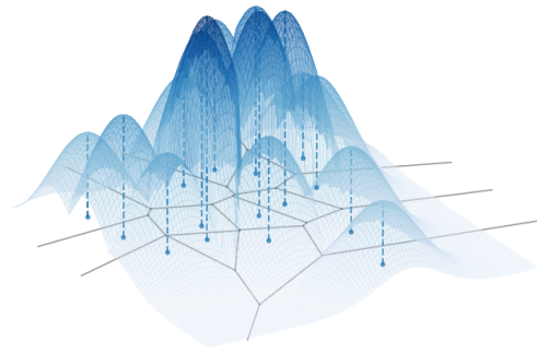
Figure 1: Graph of a density estimated by the CVDE, with the Voronoi tessellation underneath.
