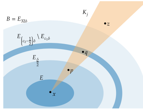
Figure 9: Graphical depiction of sets and points appearing in the proof of Proposition D.3.
